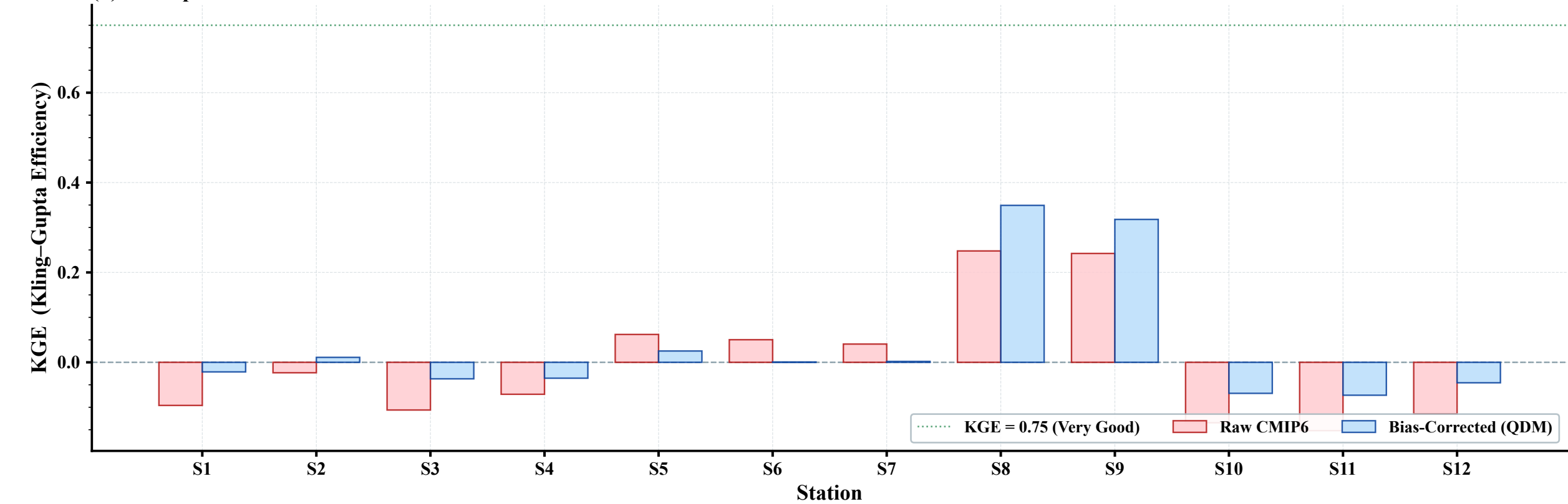
(b) KGE per Station — Ensemble Mean: Raw vs Bias-Corrected
